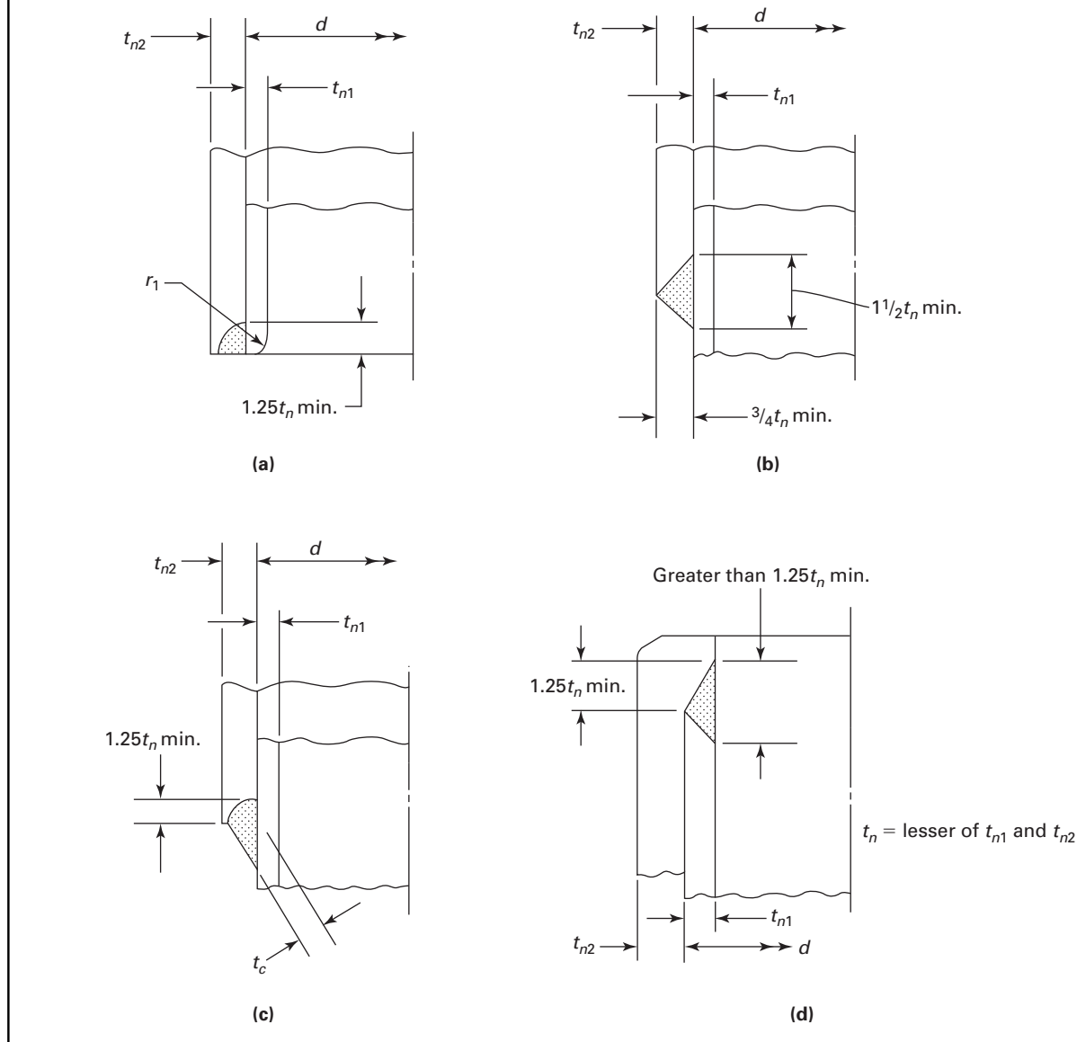
Figure NB-4244(d)-2 Partial Penetration Nozzle for Coaxial Cylinders
