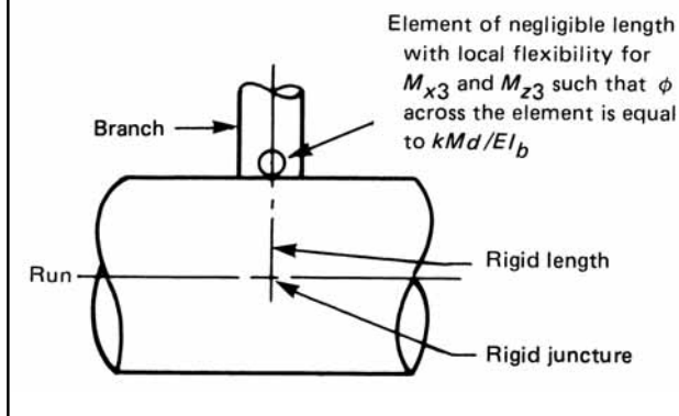
Figure NB-3686.5-1 Branch Connections in Straight Pipe
