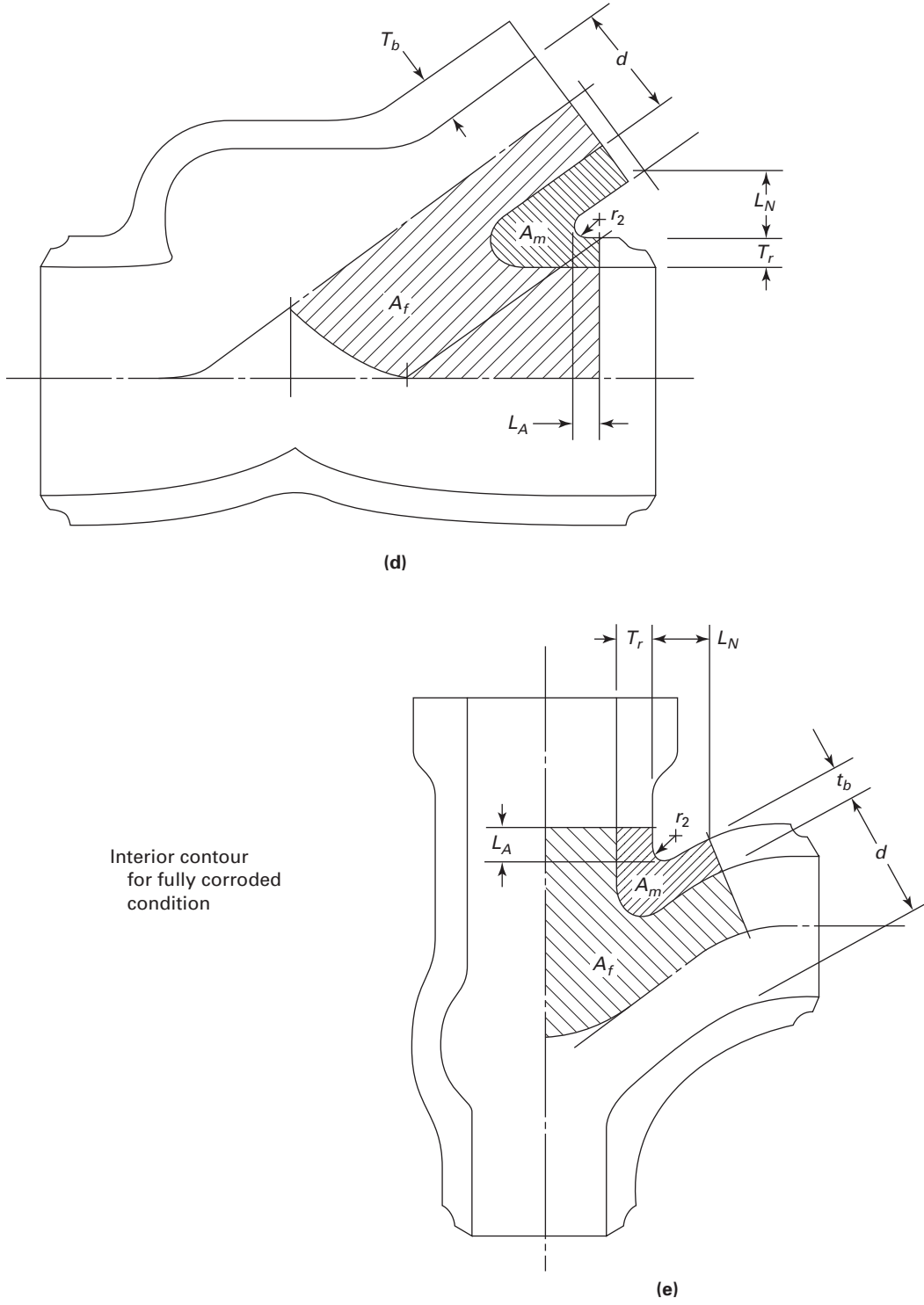
Figure NB-3545.1(a)-1 Pressure Area Method (Cont'd)
