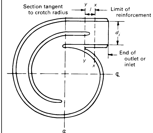
Figure NB-3433.4-1 Minimum Tangential Inlet and Outlet Wall Thickness
