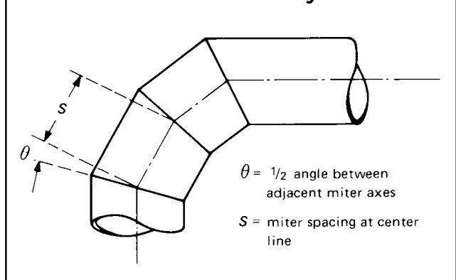
Figure NB-3644(b)-1 Miter Joint Geometry
