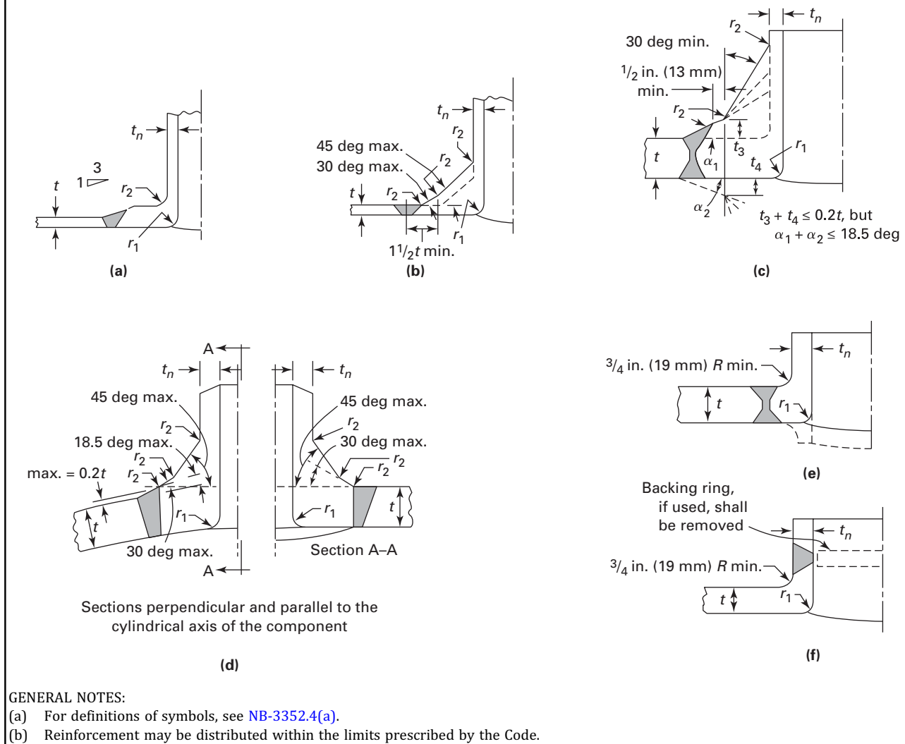
Figure NB-4244(a)-1 Nozzles Joined by Full Penetration Butt Welds
