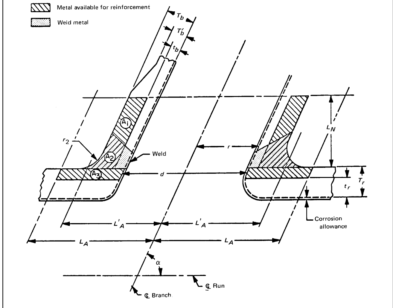
Figure NB-3643.3(a)-2 Typical Reinforcement of Openings
