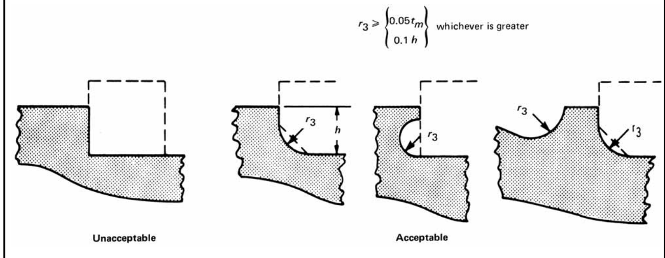
Figure NB-3544.1(c)-1 Ring Grooves
