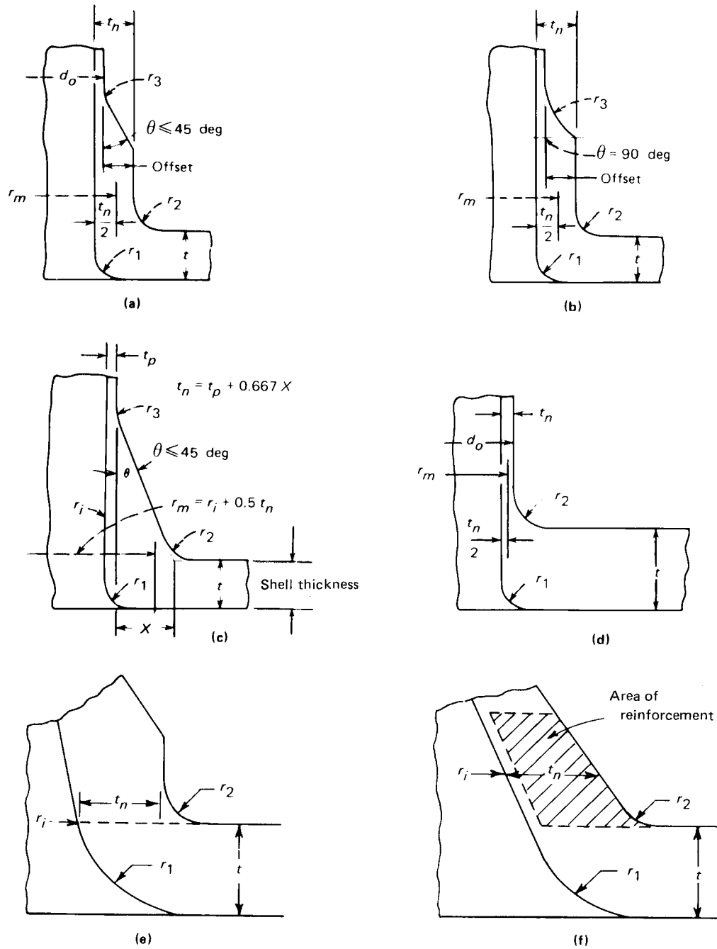
Figure NB-3338.2(a)-2 Nozzle Dimensions
