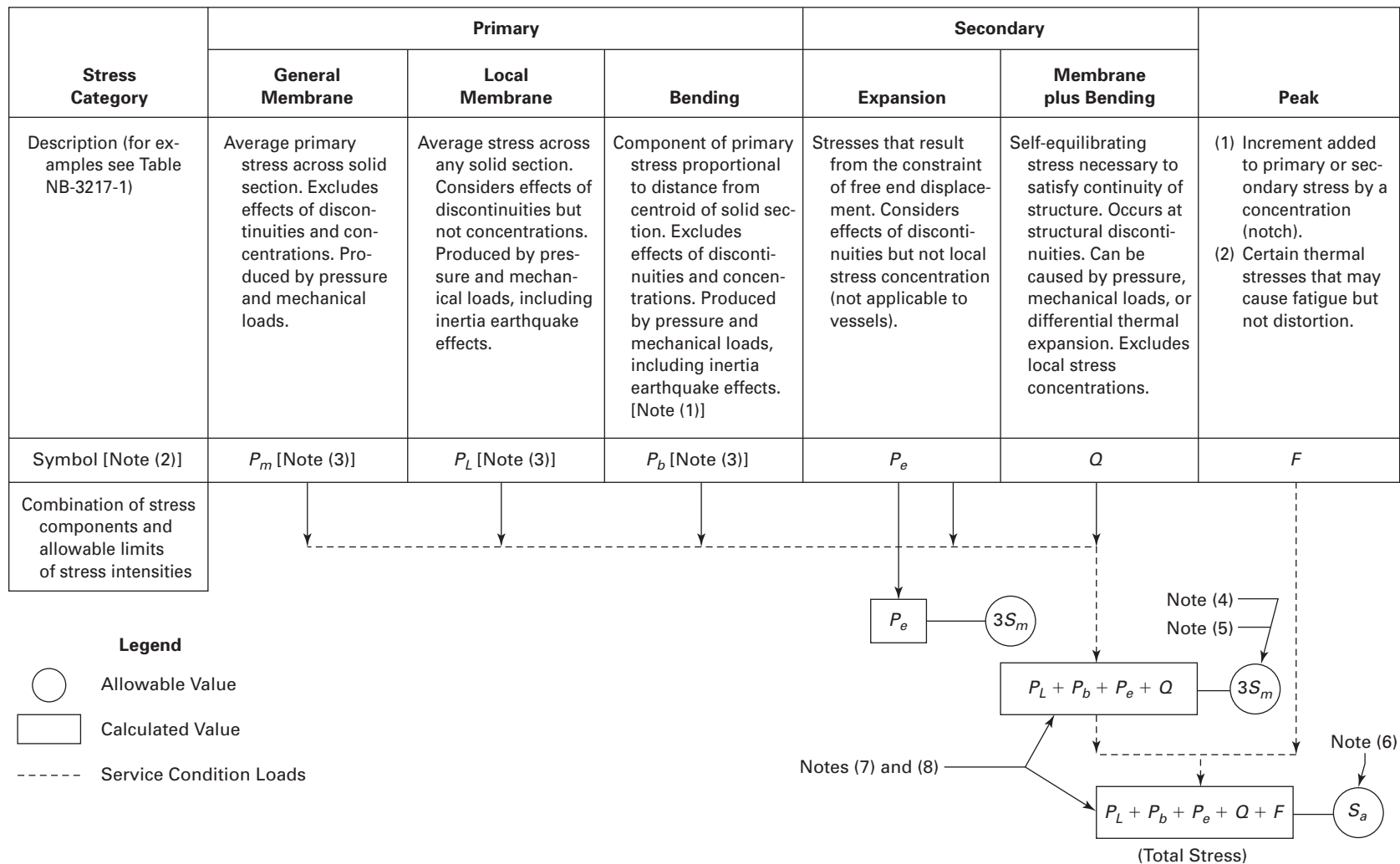
Figure NB-3222-1 Stress Categories and Limits of Stress Intensity for Level A and Level B Service Limits
