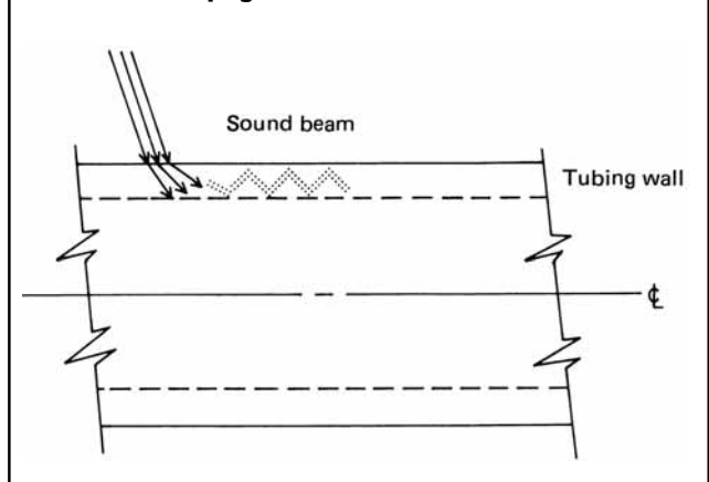
Figure NB-2552-1 Axial Propagation of Sound in Tube Wall
