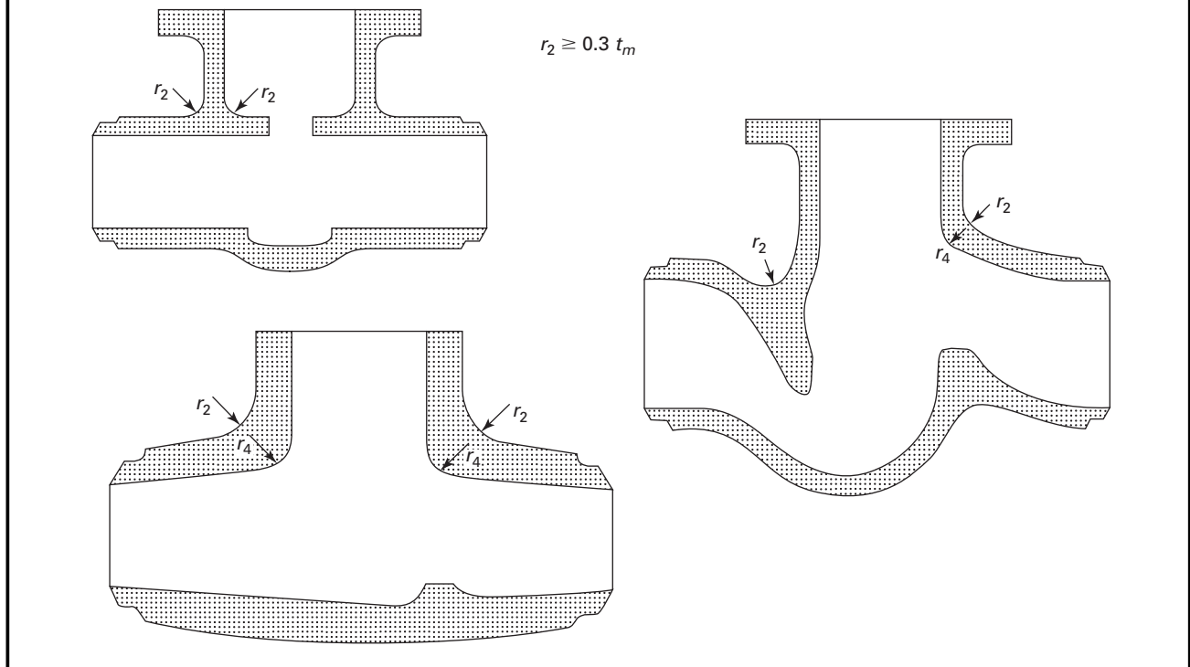
Figure NB-3544.1(a)-1 Filletlets and Corners
